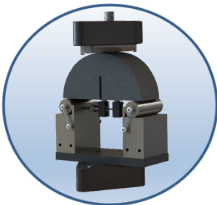
Semi-Circular Bending (I-FIT)
